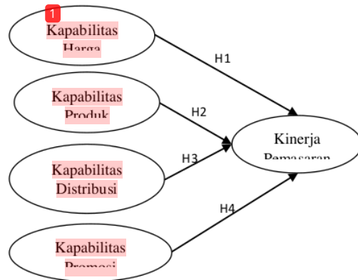
Gambar 1. Model Penelitian
